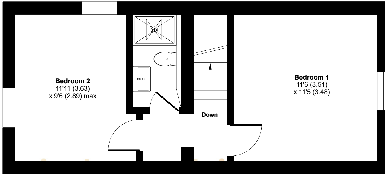
FIRST FLOOR
